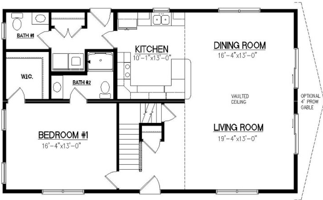
First Floor (w/ Basement)
